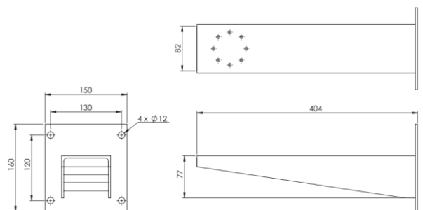
WB-SS1CH - Wall Bracket Outline Dimensions
